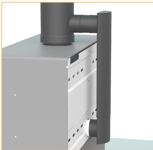
Snorkel connection
