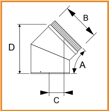
Stove pipe elbow VF-3-60-145
