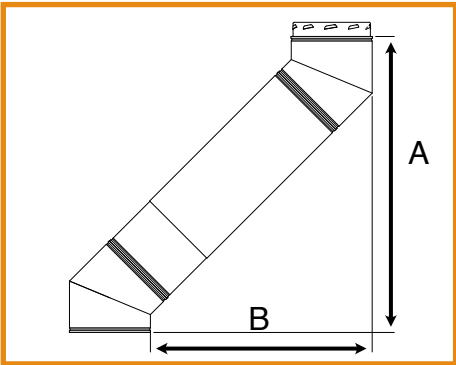
Adjustable length between elbows
