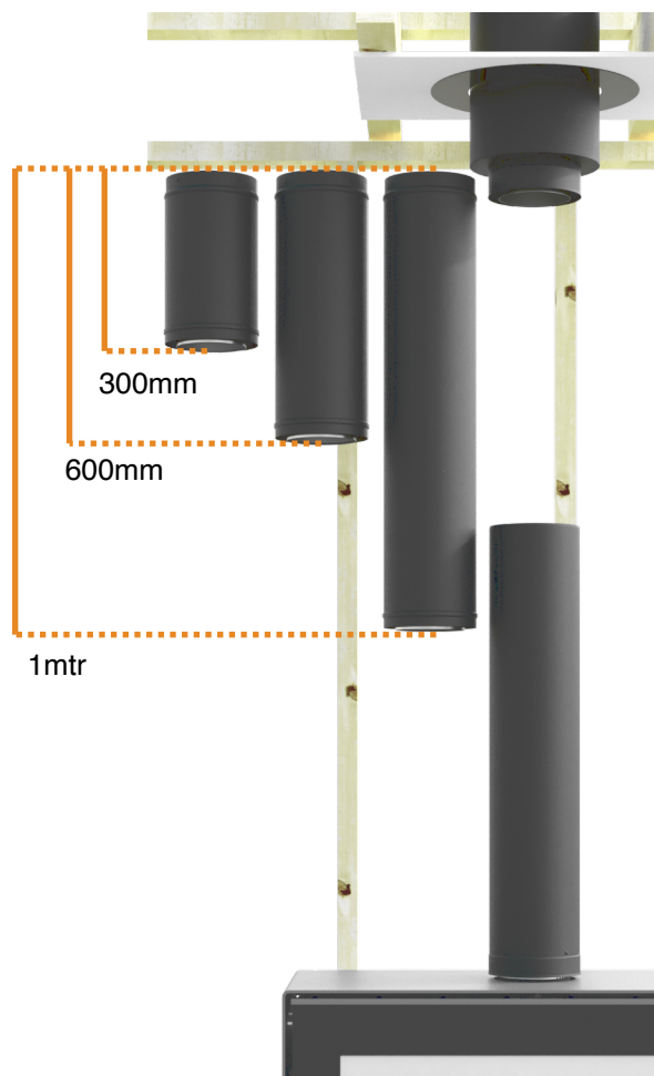
Adjustable female addition example
