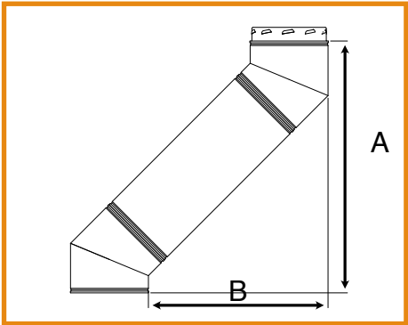
Fixed length between safety vent elbows
