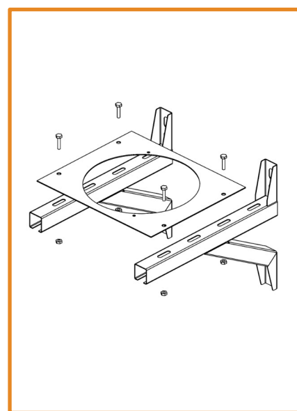
VL6SB-02-FI EXTERNAL WALL BRACKET
