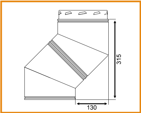
Back to back elbows
